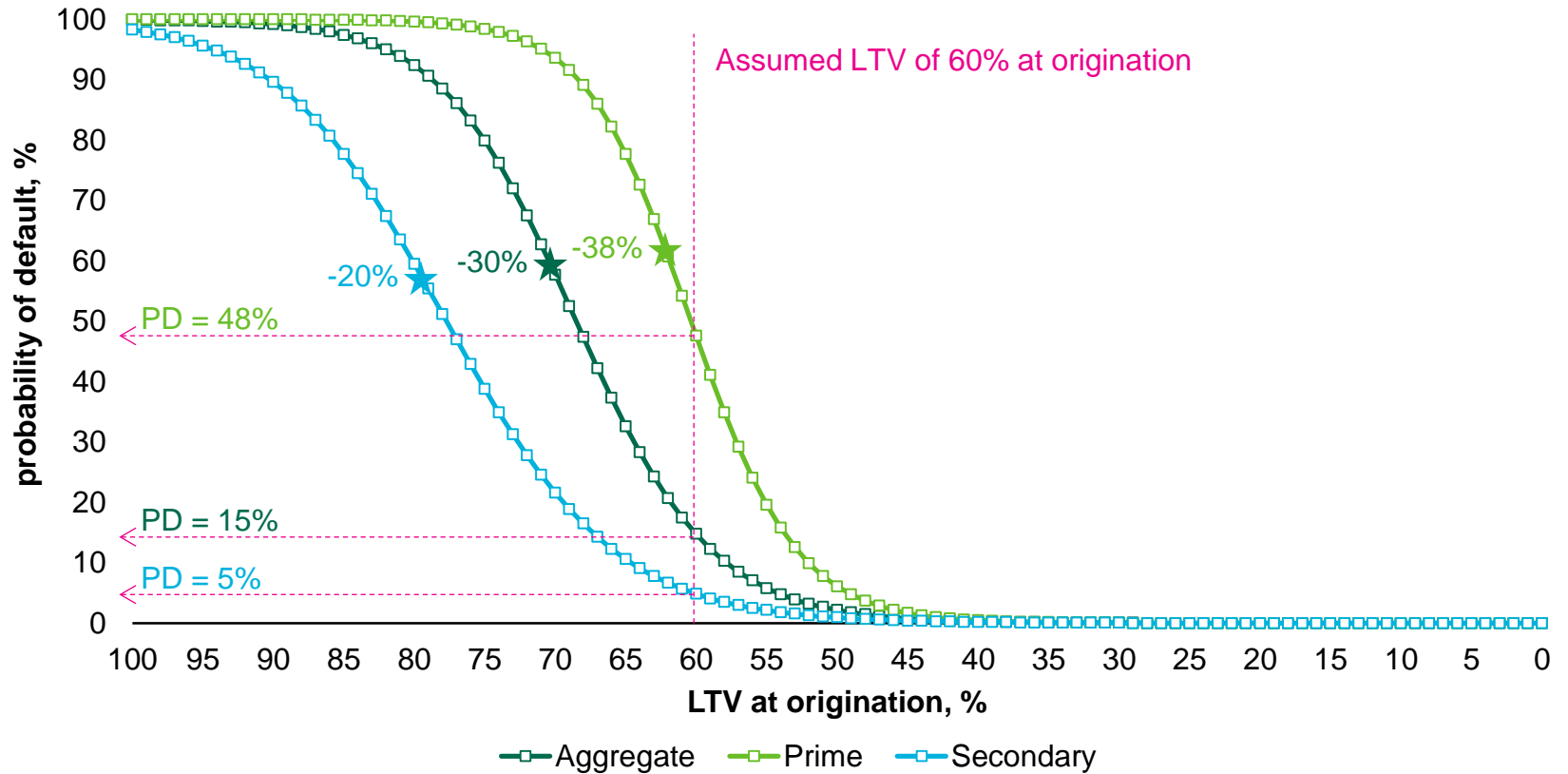
Figure 3: Probability distributions for BoE Stress scenario for 2015 lending
